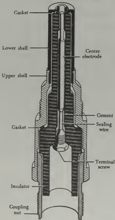
FIGURE 4-78. Typical annular-gap igniter plug.
